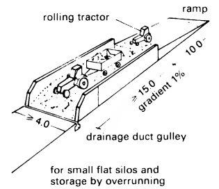
11 Flat silo with ramp
